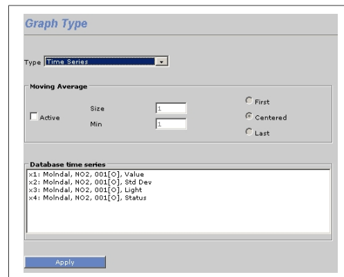
Figure 3.4.1 Graph type.
