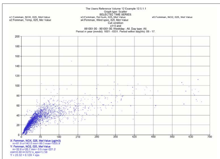
Figure 3.5.1.1 Scatter plot of NO 2 vs. NO x concentrations.
