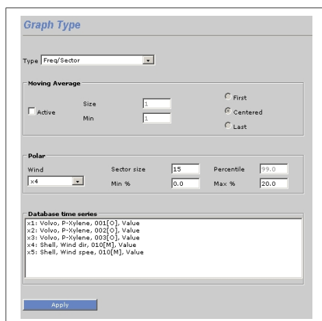
Figure 3.4.3.8 Graph Type frame with settings for a wind rose in the Polar sub frame.
