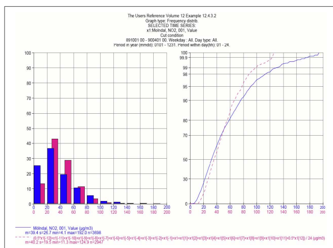
Figure 3.4.3.4 Frequency distribution graph with percentage histogram and cumulative distribution chart. The effect of applying a 24-h moving average can be seen by comparing plot variable 1 and 2.
