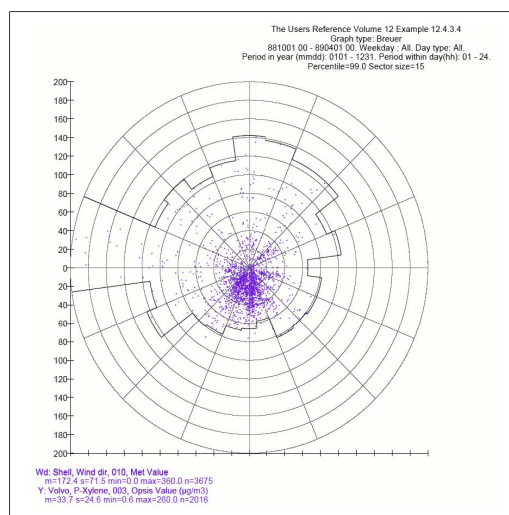
Figure 3.4.3.6 Breuer diagram with P-Xylene concentrations contra wind direction in a polar coordinate system. The 99%-ile concentration in each sector is indicated by an arc.
