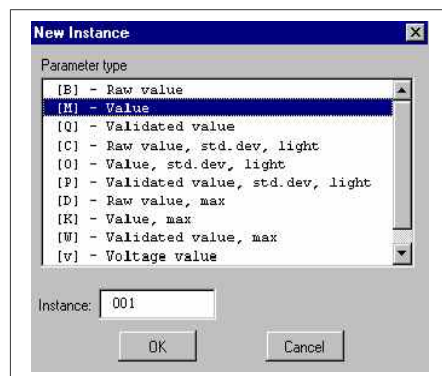
Figure 3C.6. New instance.
