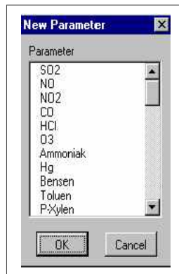
Figure 3C.5. New parameter.
