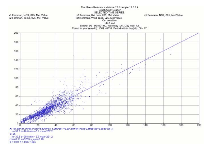
Figure 3.5.1.7 Scatter plot of measured contra estimated NO 2 concentrations.
