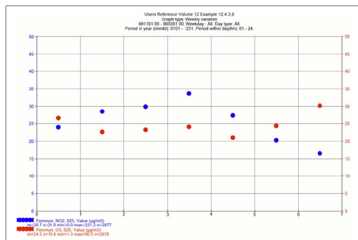
Figure 3.4.3.10 Weekly variation diagram with anticorrelated \text{NO}_2 and ozone concentrations. During weekends, the \text{NO}_2 concentration is lower than during weekdays.
