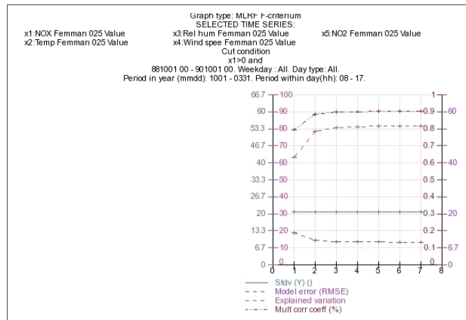
Figure 3.5.1.6 Regression model performance for cross validated models.
