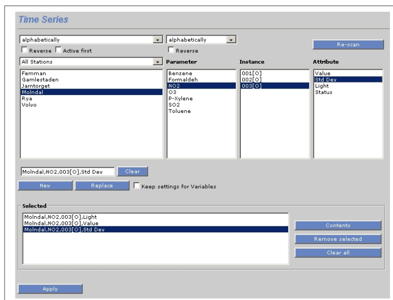
Figure 3.2.3.2 Time Series frame with available stations and parameters in the REF database with 1 hour resolution. Up to 64 time series can be selected for further processing.
